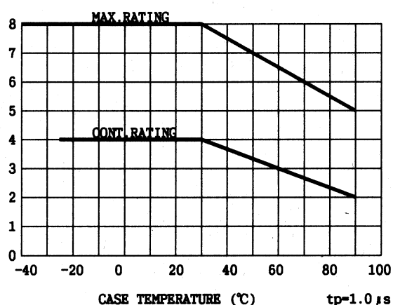
FIG.1 RF INPUT POWER MAXIMUM AND CONTINUOUS RATINGS tp=1.0 µs
