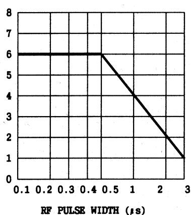
FIG.2 PULSE WIDTH DEPENDENCE OF CONTINUOUS RATINGS at-25°C
